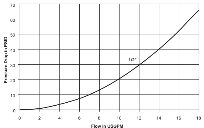
5000 Series (1/2") Test Fluid: Oil - 200 SUS
