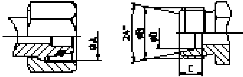
with O-ring
